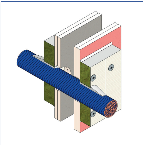
FS712 Intucoat Brush applied to raw edge of pattern fit/surface mounted FB750 Intubatt
