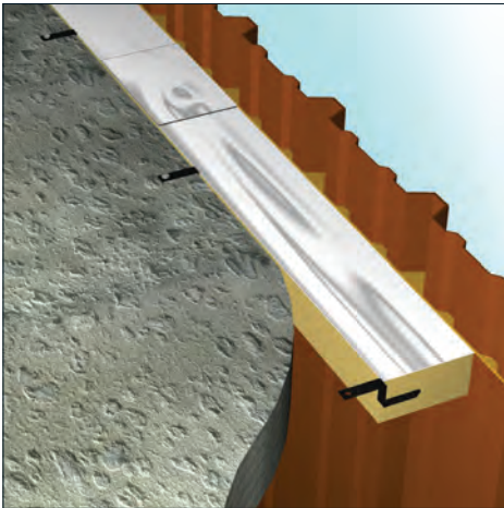
FJ240 with Z-clips on a steel profile cladding
