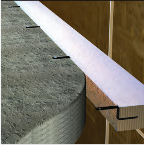
FJ240 with Z-clips on a non-combustible curtain wall
