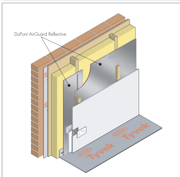
Figure 1 Typical wall and floor installation
