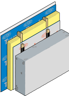
Fig. 10 Masonry wall Internal insulation upgrade
