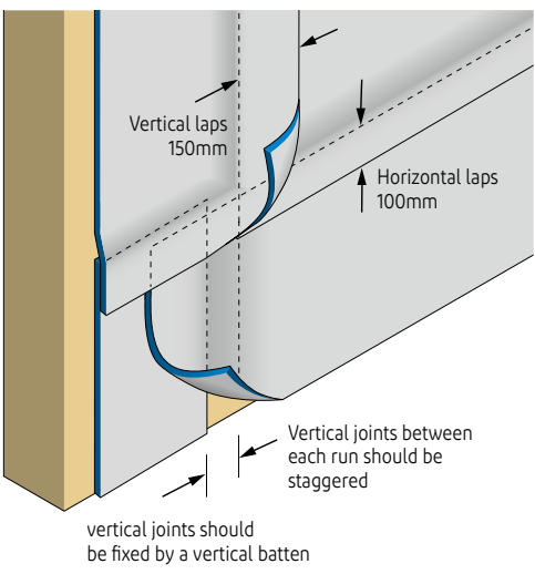
Fig. 14 - Horizontal and vertical laps
