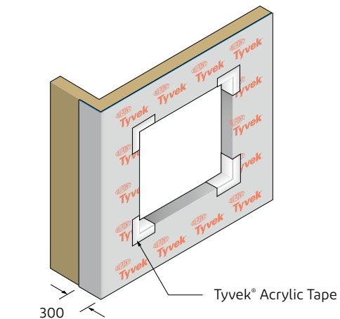
Fig. 17 - External corner and window opening
