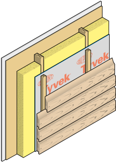
Fig. 4 Timber Frame Reverse construction) Horizontal Weatherboarding
