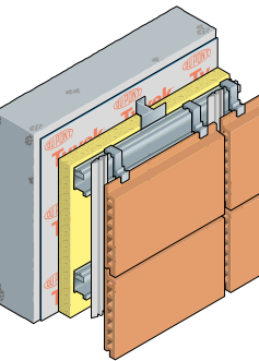
Fig. 11 Masonry wall Rainscreen cladding
