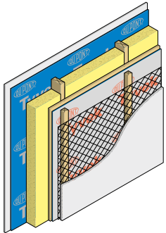
Fig. 7 Timber Frame Cement render on lathe
