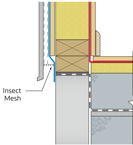
Fig. 19 - Base detail (render & lathe)
