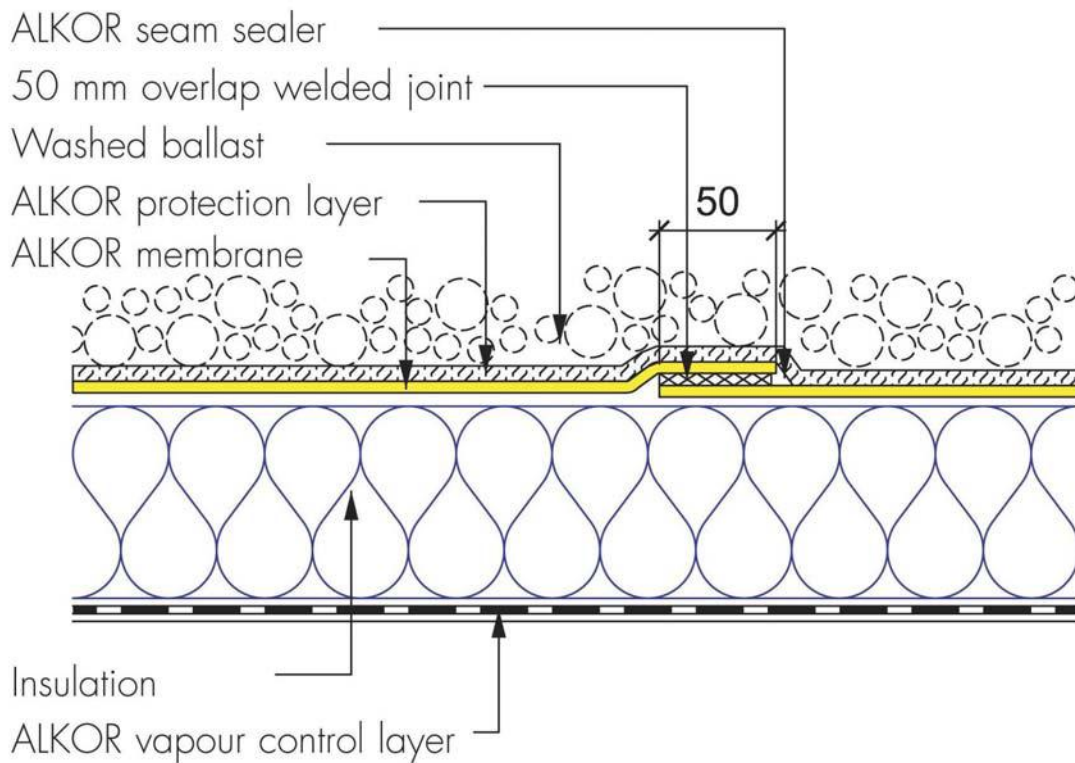
Figure 2: Loose Laid Ballasted Seam
